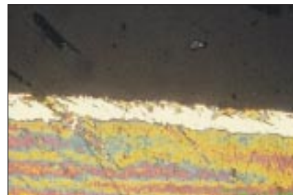
Figure 4 - 9ct gold-silver alloy treated 7 h at 165°C in alum paste. x250
