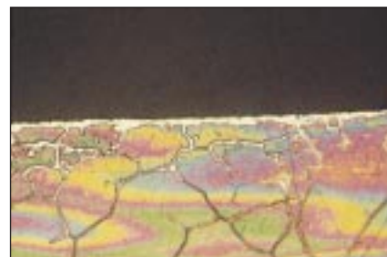
Figure 5 - 9ct gold-silver alloy treated 15 minutes at 600°C in alum paste. x250
