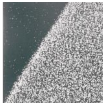
Figure 6 - EPMA analysis showing gold distribution inwards from the surface of 9ct gold-silver alloy given 9 cycles of torch heating in alum paste and brick dust.
