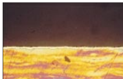
Figure 11 - 9ct gold-silver-copper alloy heated 2h in a boiling solution of alum. x400
