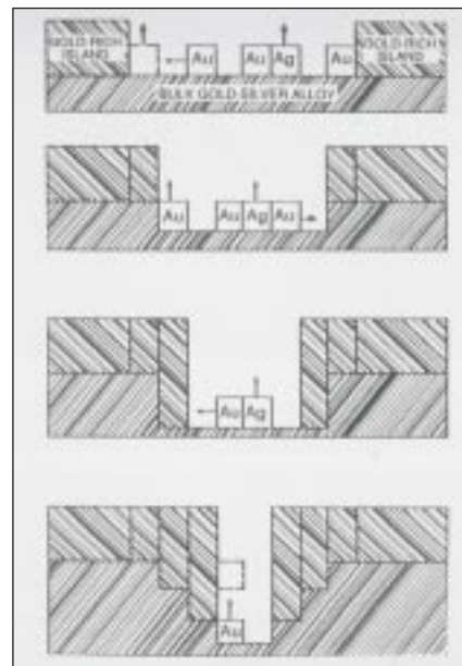
Figure 14 - Corrosion and diffusion re-ordering model by selective dissolution. After Forty et al (15,16)
