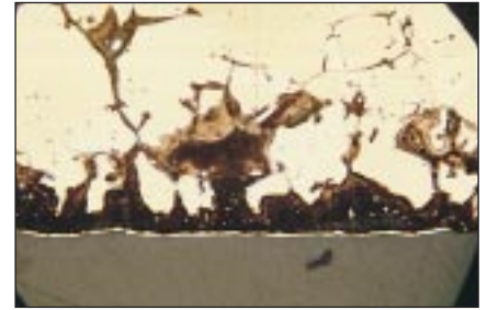
Figure 2 - Cross-section of Vicus disc showing depletion gilded layer. x200
