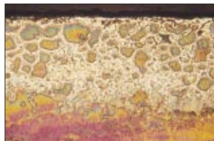
Figure 10 - 9ct gold-silver-copper alloy heated 14 h at 450°C in alum paste and brick dust. x200
