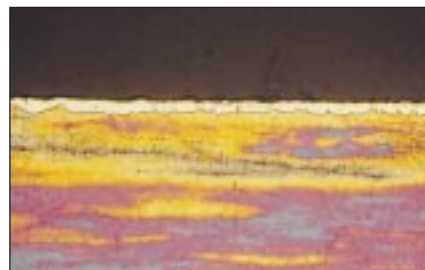
Figure 12 - 9ct gold-silver-copper alloy given 9 cycles of torch heating in alum paste and brick dust. x400
